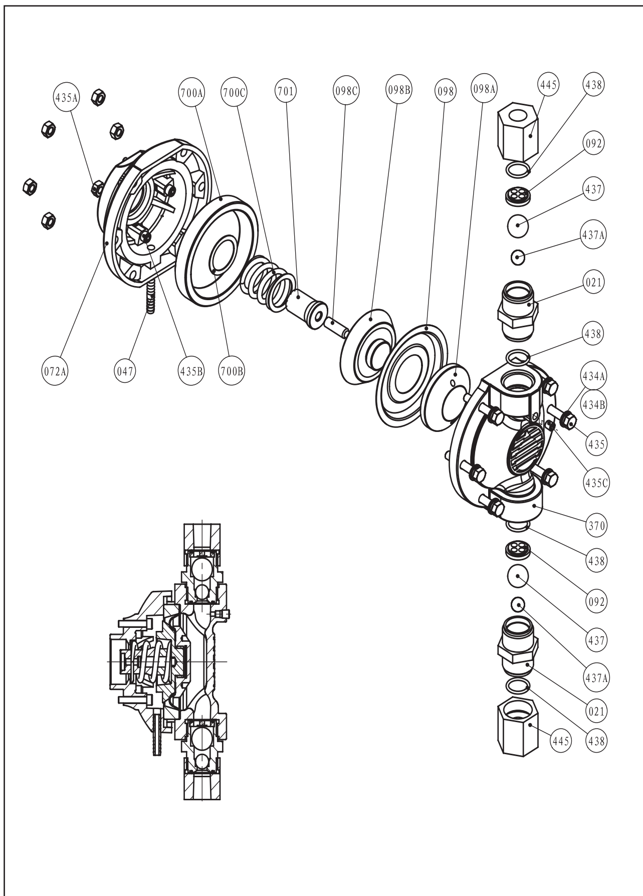
图5-15 GM0090~GM0500 不锈钢和浆料液力端
